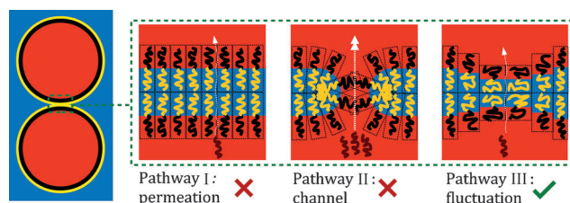
Figure 3. Three microscopic pathways for contact ripening. Pathway I consists in the non-correlated permeation of oil molecules across an unperturbed bilayer. Pathway II corresponds to the opening of large channels in the surfactant films allowing several oil molecules to go through. Pathway III corresponds to a synchronous decrease in the thickness of both hydrophilic and hydrophobic surfactant layers, with a correlated increase in the area per surfactant molecule. The resulting local thinning and disordering of the surfactant layer favors the oil transfer between droplets. Only pathway III is consistent with the data from Figure 4.
